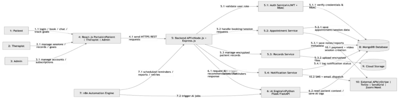
Fig 2.4 Collaboration Diagram
