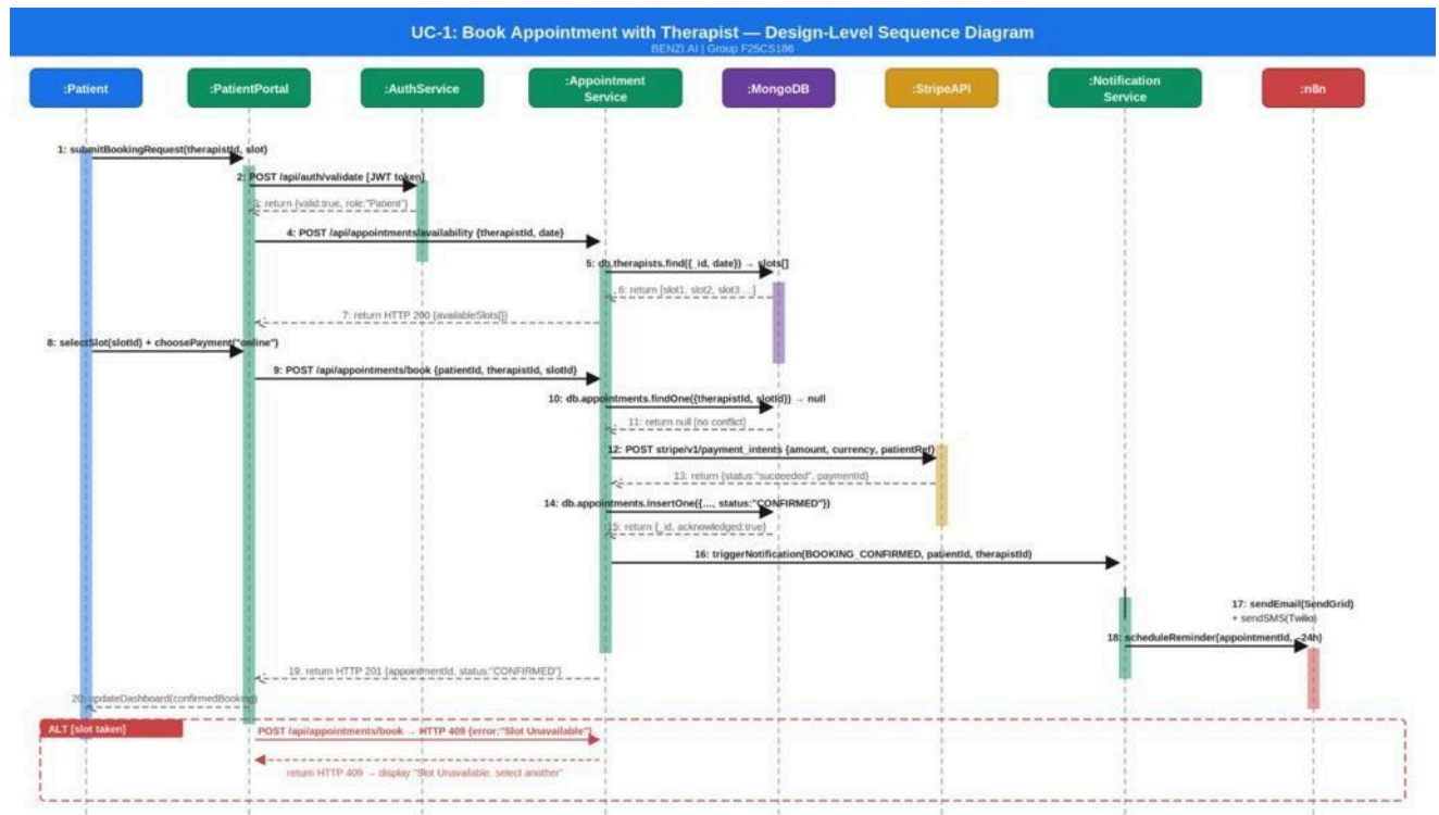
Figure 1: UC 1 Book Appointment Design Level Sequence Diagram
