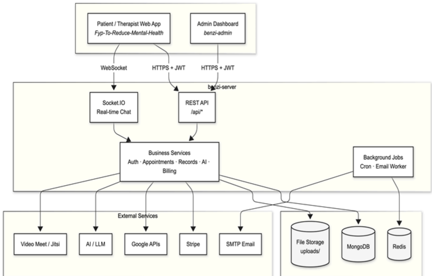
Fig 2.2 Component Diagram
