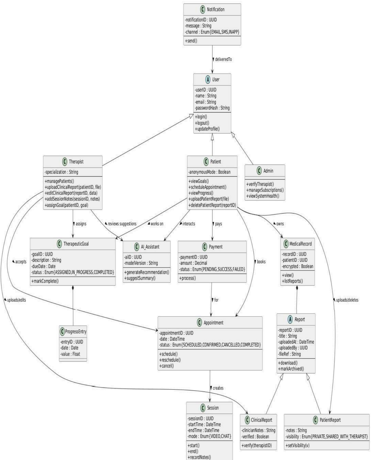
Fig 3.2 Abstract Diagram
