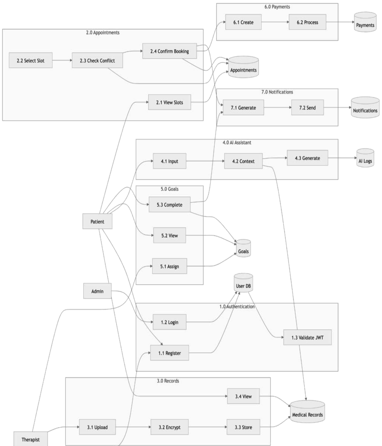
Fig 3.5 Level 2 DFD
