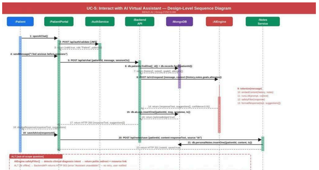
Figure 5: UC 5 AI Virtual Assistant Interaction Design Level Sequence Diagram
