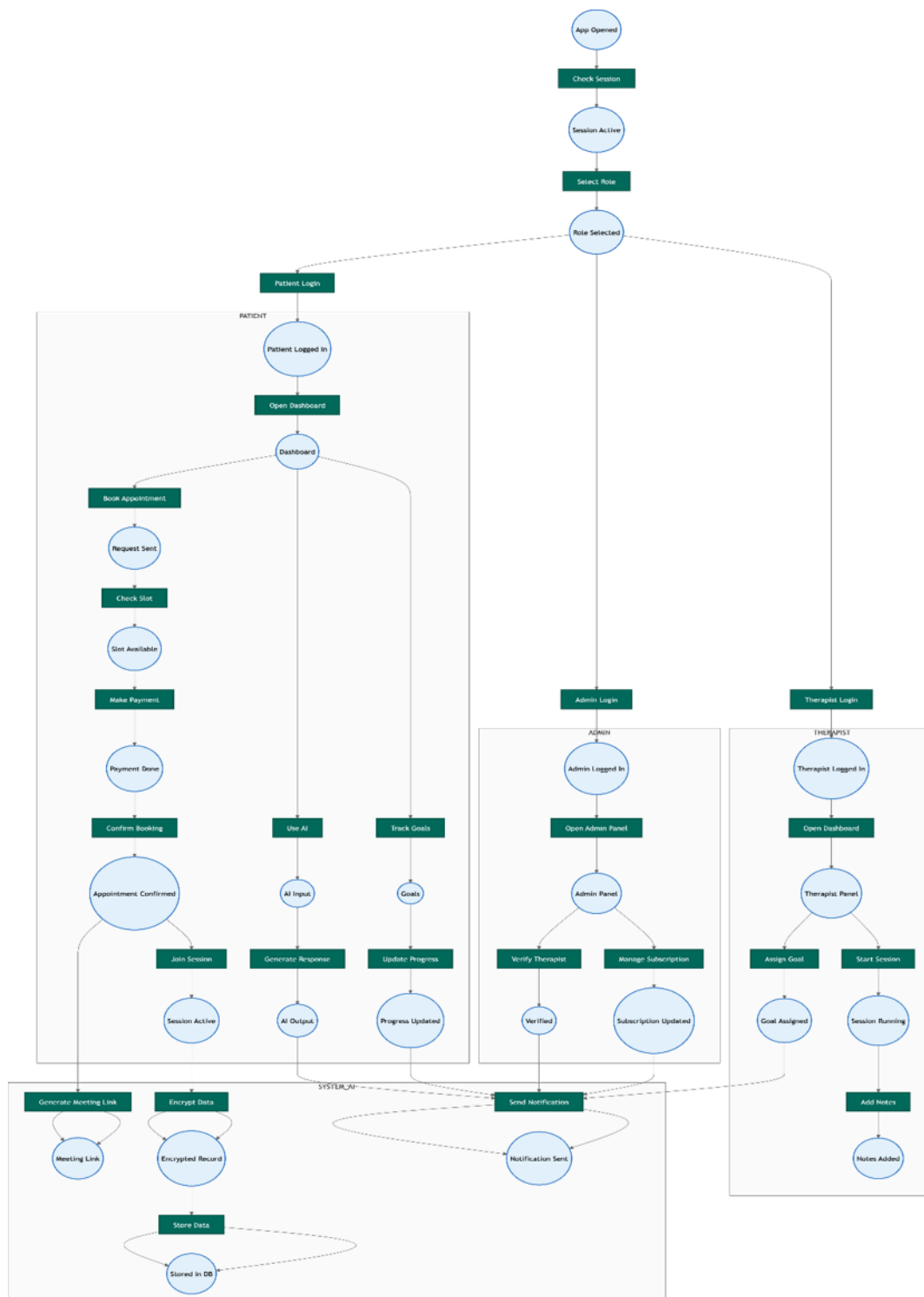
Fig 5.4 Petrinet Diagram
